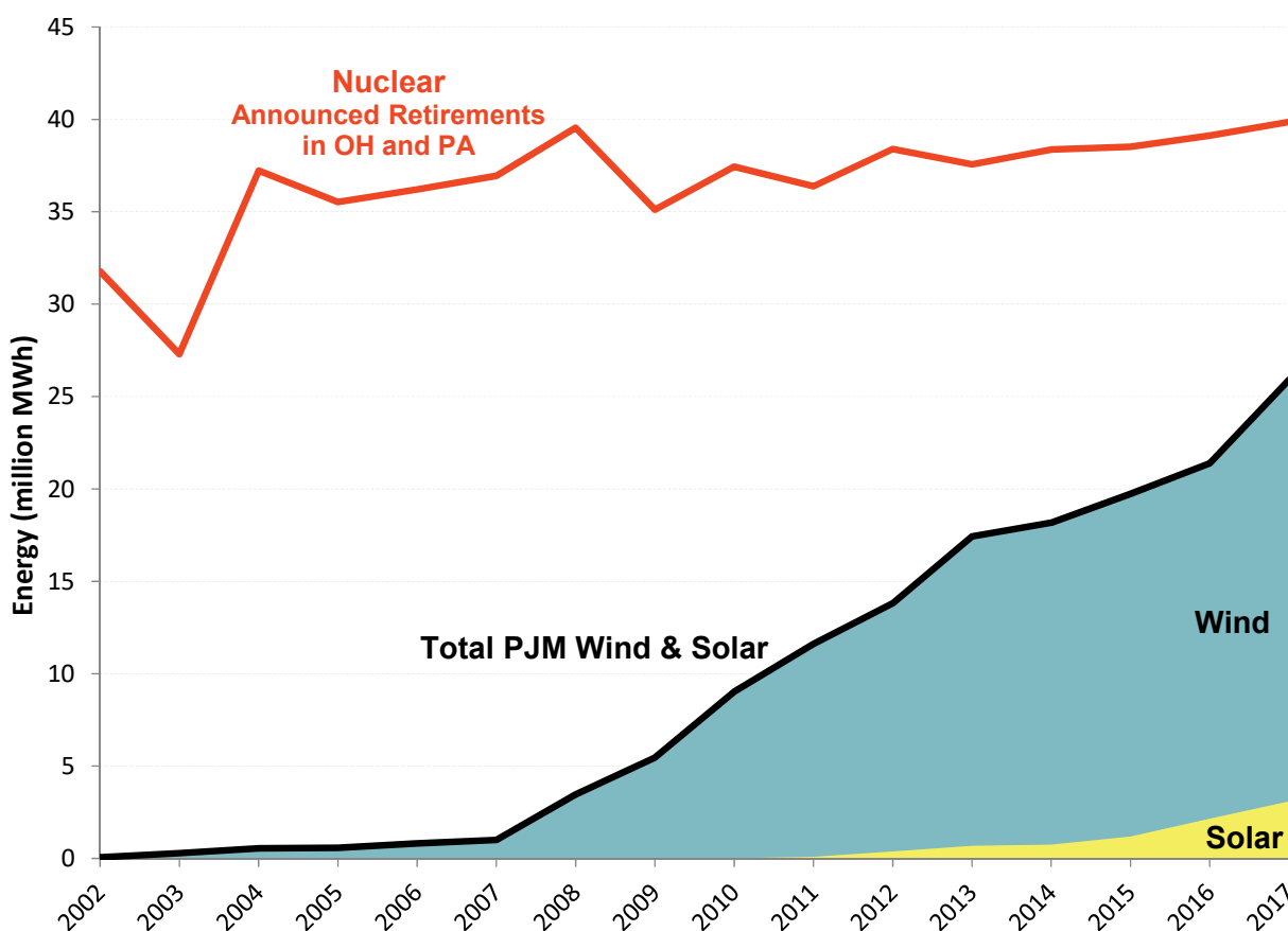
Figure 1: Generation of Ohio and Pennsylvania Nuclear Plants with Announced Retirements vs. Total PJM Renewable Generation
